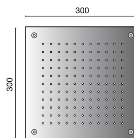
NK LOGIC Rociador encastre techo Square 30 cm. Ceiling mounted Square 30 cm rain shower head. espejo - mirror 100090737 - N186490003
