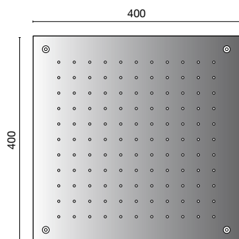
NK LOGIC Rociador encastre techo Square 40 cm. Ceiling mounted Square 40 cm rain shower head. espejo - mirror 100090738 - N186490002
