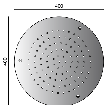
BELA Rociador encastre techo Rondo 40 cm. Ceiling mounted Rondo 40 cm rain shower head. espejo - mirror 100090721 - N185709903
